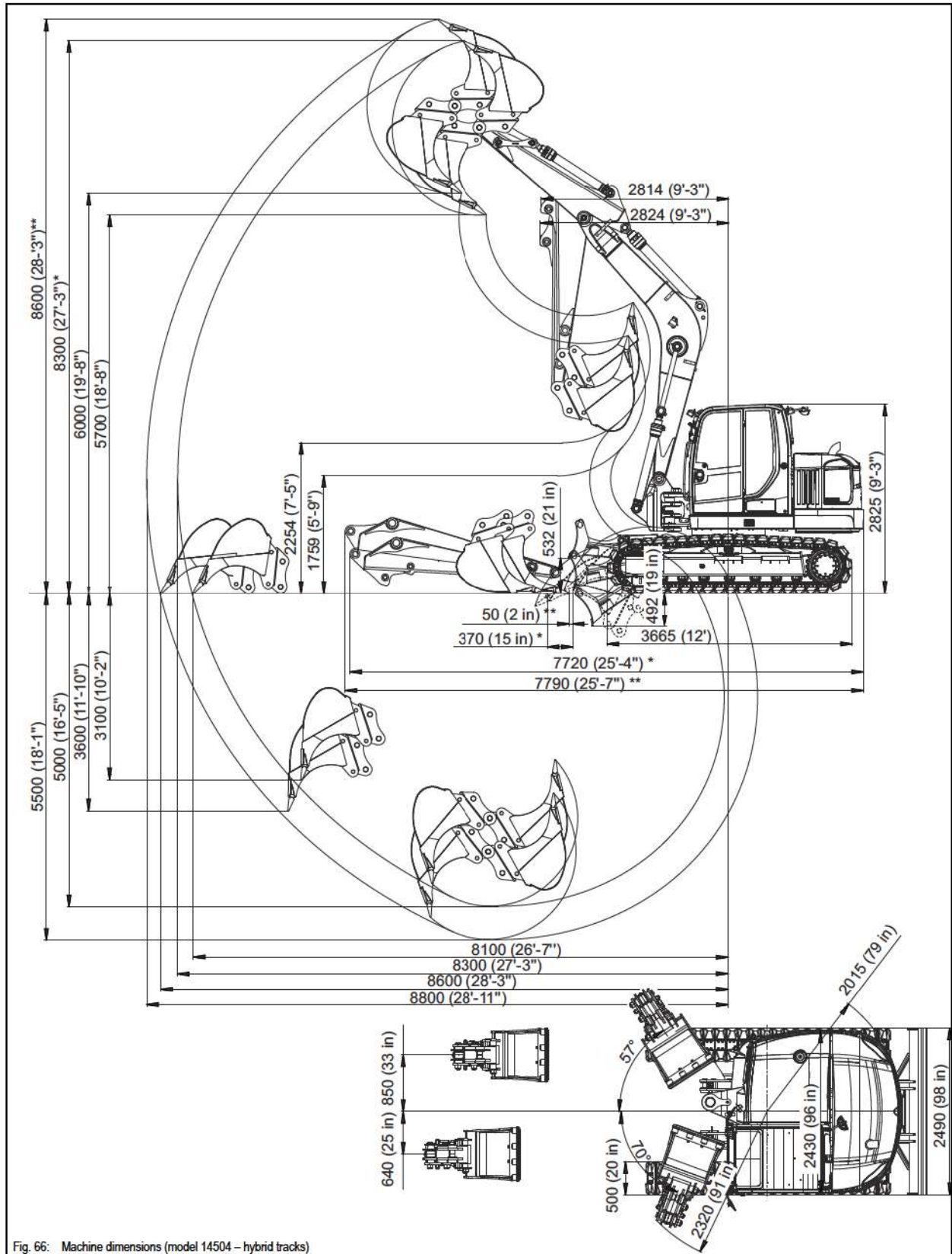
Fig. 66: Machine dimensions (model 14504 – hybrid tracks)
